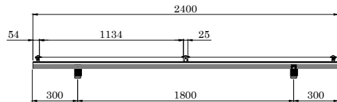
VISTA FRONTAL
