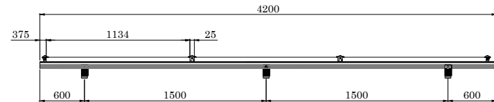
VISTA FRONTAL
