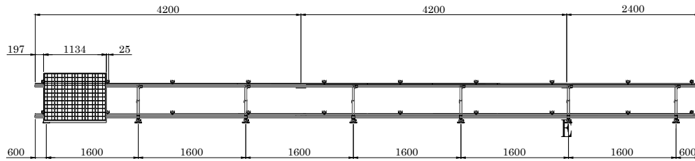
VISTA FRONTAL
